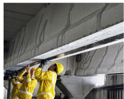
CRACK PREVENTION/REDUCTION
