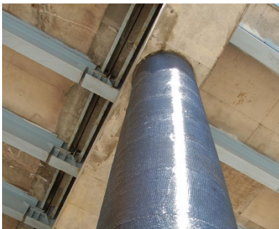
COLUMN STRENGTHENING
