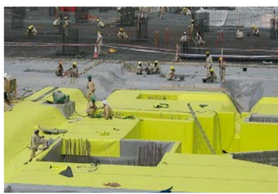
Membranes for basement waterproofing
